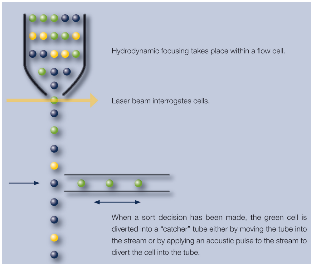
Figure 2. Mechanical Sorting
