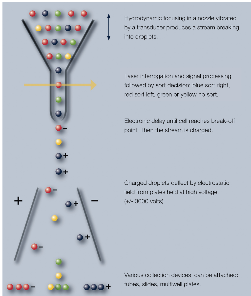
Figure 1. Electrostatic Sorting
