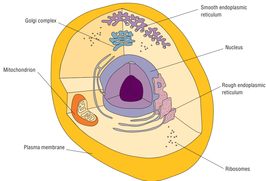
Figure 1. The Cell
