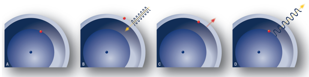
Figure 1. A) Electrons in an atom (red) are normally found at their ground state. B) When an electron is excited by high-energy light, such as ultraviolet light, the electron moves from the ground state to a higher energy state. C) The electron is unable to sustain the higher energy state and quickly drops to the lowest singlet excited state. The energy lost is given off as heat. The amount of energy lost determines the Stokes shift. D) The electron then falls back to its ground state, and energy is emitted as light with a longer wavelength and less energy than the light that excited the electron.
